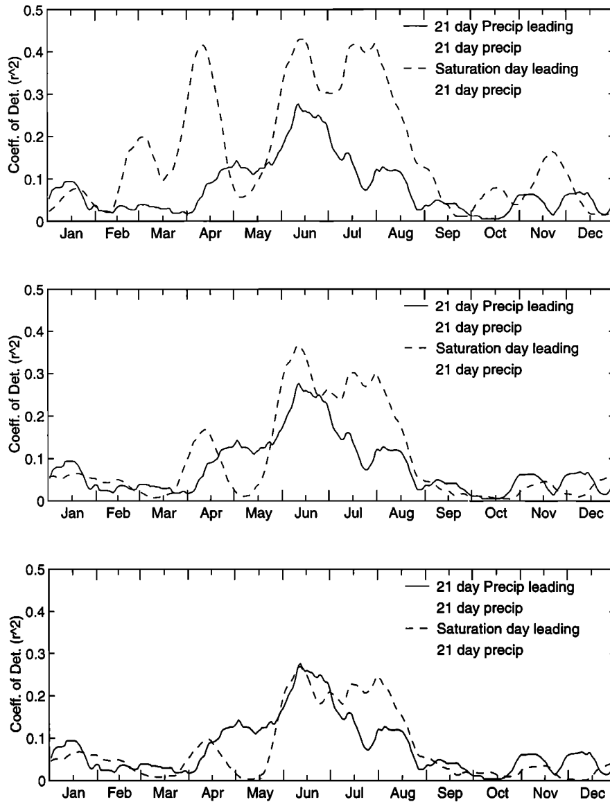
Figure 7. Comparison of smoothed lines of the correlation between adjacent precipitation windows (top) top 10 cm, (middle) top 50 cm, and (bottom) top 90 cm) (solid line, from Figure 5) and of the correlation between soil saturation and subsequent precipitation (dashed line, from Figure 4).
