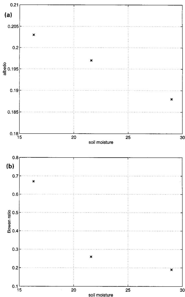
Figure 3. Observations on soil moisture (volume of water per bulk volume of soil) and on (a) albedo and (b) Bowen ratio during FIFE. The data are averaged into three categories using three bins of similar soil moisture conditions; each bin contains an equal number of data points.
