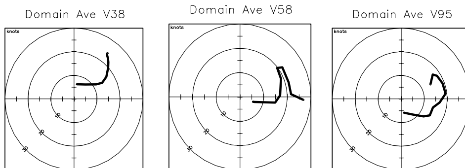
Figure 10. Hodographs to 300 mbar above ground surface (AGS) for three cases in the wet soil advantage regime where reduction of the initial and boundary winds increased the convective activity. In all three cases the winds back with height, and in all three cases, convective activity was greater in the reduced-winds runs than in the observed winds runs. See text for more information.
