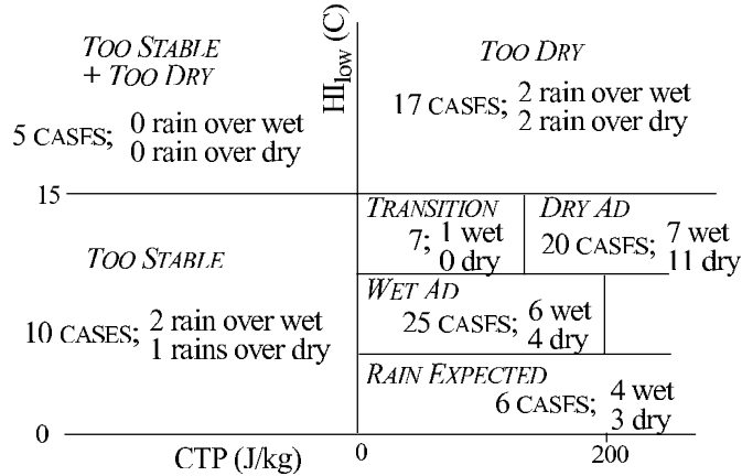
Figure 3. Number of case studies with CTP and HI_{low} characteristics in each of the regimes from Figure 1. (a) Simulations with original initial and boundary winds (supplied by Eta Model data). (b) Simulations with initial and boundary winds reduced to 10% of original values. These simulations were only run for cases that were not extremely dry and/or stable (very near the boundaries with other regimes). Wet Ad and Dry Ad are short for wet soil and dry soil advantage regimes, respectively.
