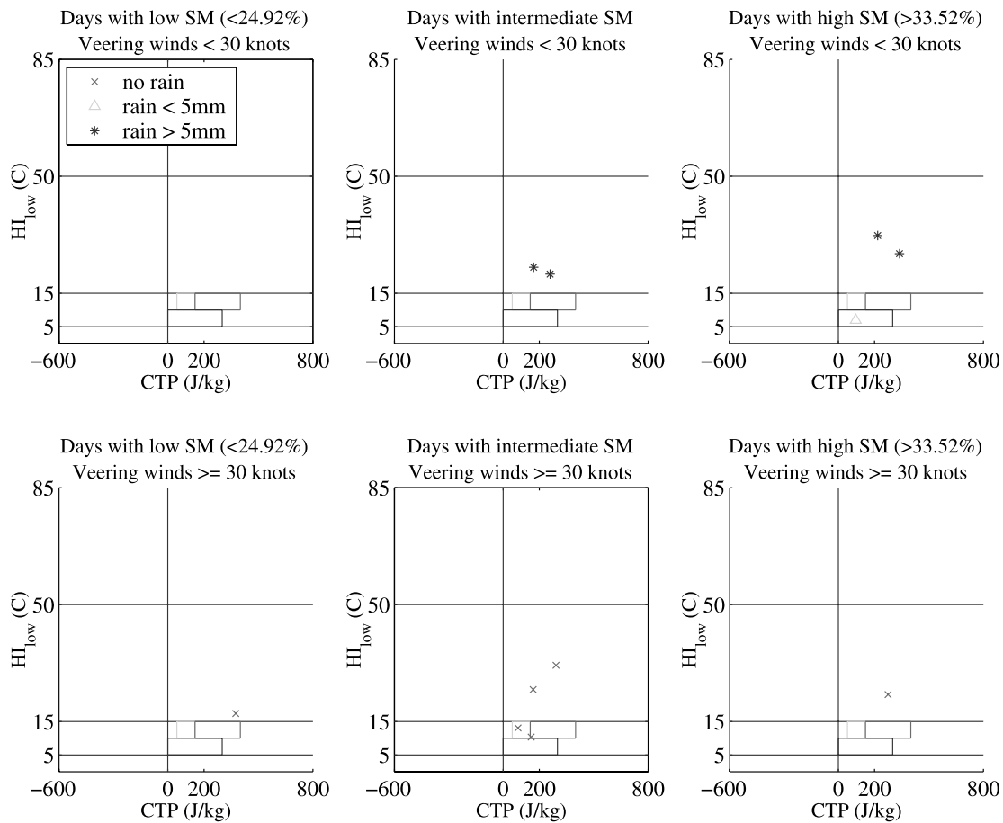
Figure 16. As in Figure 15 but only for those days with veering winds. Top row of plots is for those days with veering winds <30 knots; bottom row is for those >30 knots.
