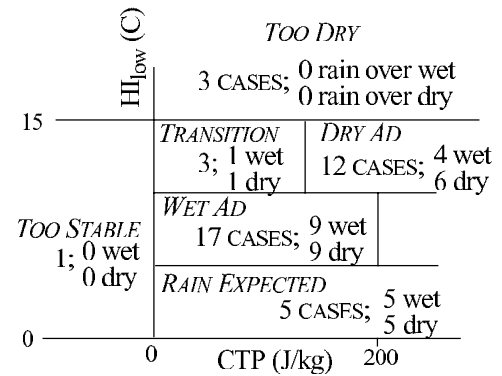
Figure 3. Number of case studies with CTP and HI_{low} characteristics in each of the regimes from Figure 1. (a) Simulations with original initial and boundary winds (supplied by Eta Model data). (b) Simulations with initial and boundary winds reduced to 10% of original values. These simulations were only run for cases that were not extremely dry and/or stable (very near the boundaries with other regimes). Wet Ad and Dry Ad are short for wet soil and dry soil advantage regimes, respectively.
