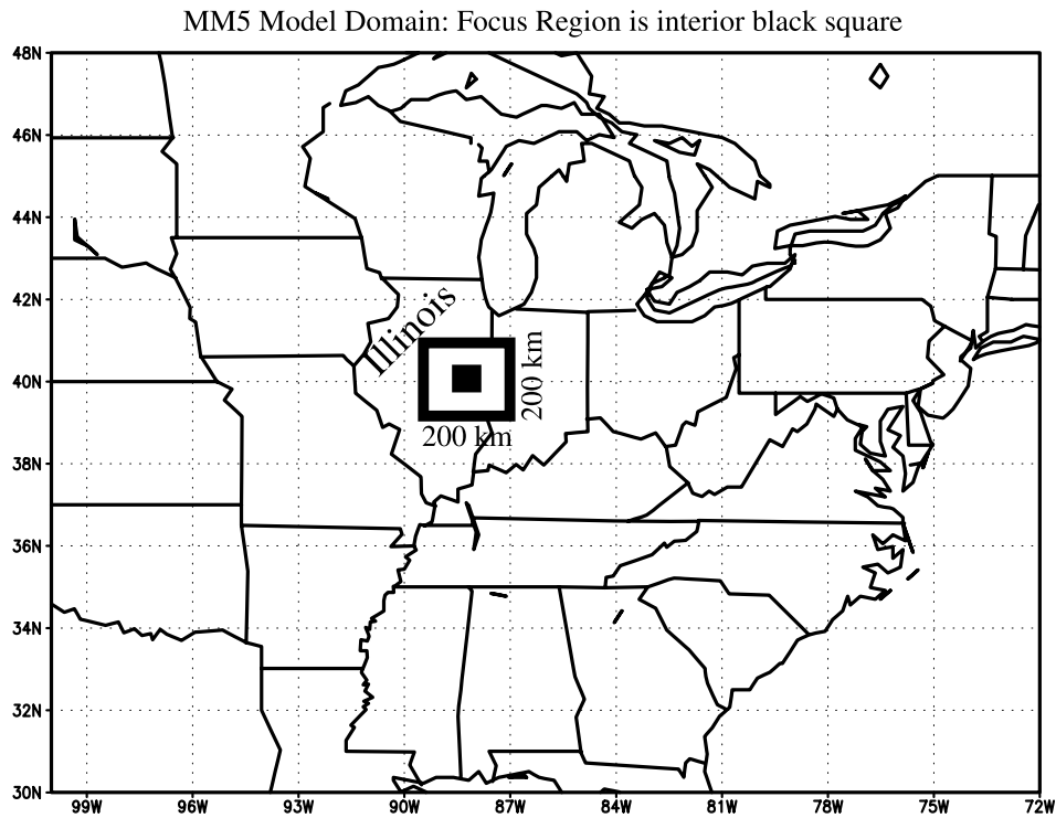
Figure 2. Model domain. Thick black line encloses full model domain ( 200 \times 200 km); solid square covers focus region ( 64 \times 64 km), which is entirely within the state of Illinois.
