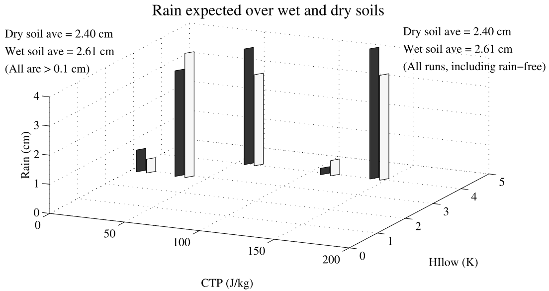
Figure 8. As in Figure 4 but for runs with reduced winds. Only five of the original six simulations were performed. Symbols in top plot are as in Figure 4.
