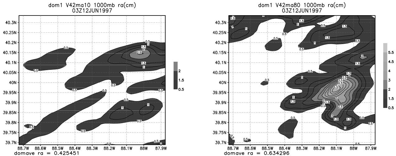
Figure 5. Total rainfall depths (cm) (left) over dry soils and (right) over wet soils in run V42 (initial sounding shown in 6; domain average CTP = 113 J/kg, HI_{low} = 3.9^{\circ}\text{C} ).
