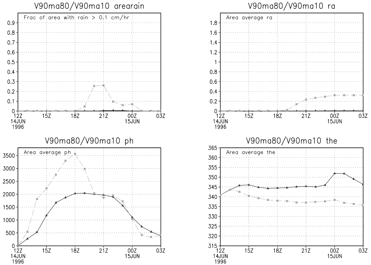
Figure 14. Time series of (top left) fractional coverage of rainfall, (top right) cumulative rainfall depth (in cm), (bottom left) planetary boundary layer height (in m), and (bottom right) surface \theta_E (in K) in the wet soil (solid lines) and dry soil (dashed light lines) simulations for case V90.
