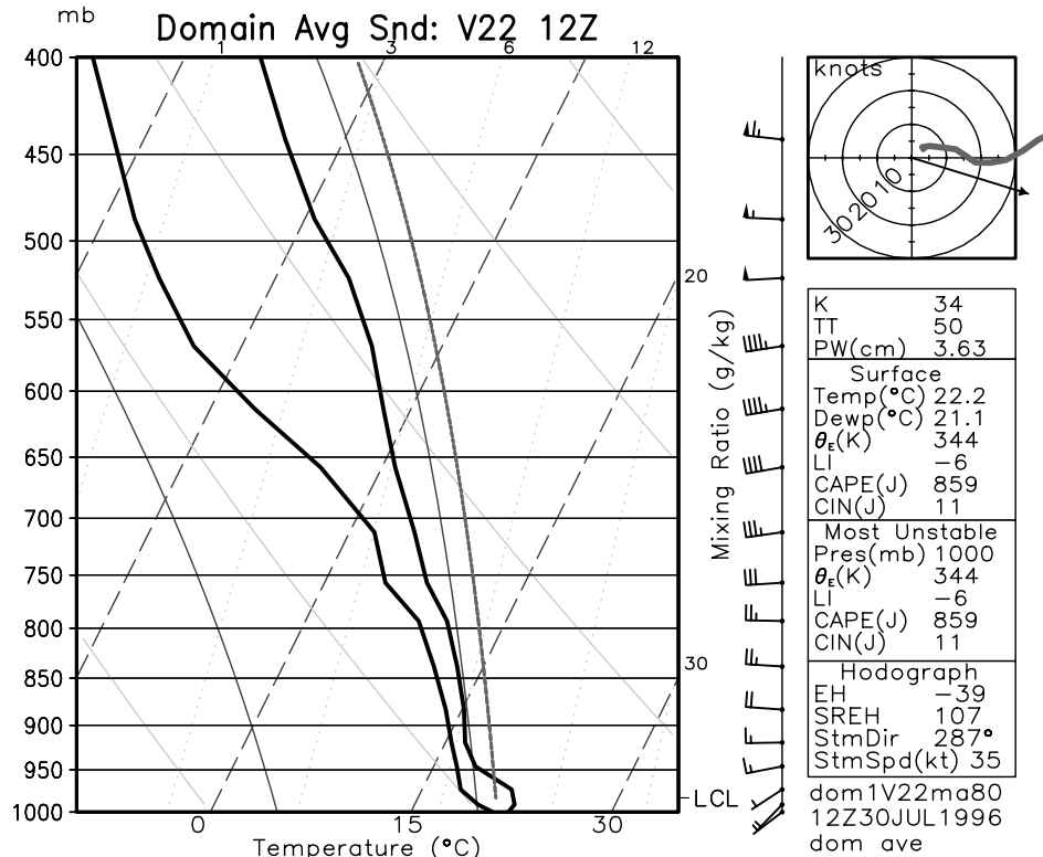
Figure 7. As in Figure 6 but for run V22.
