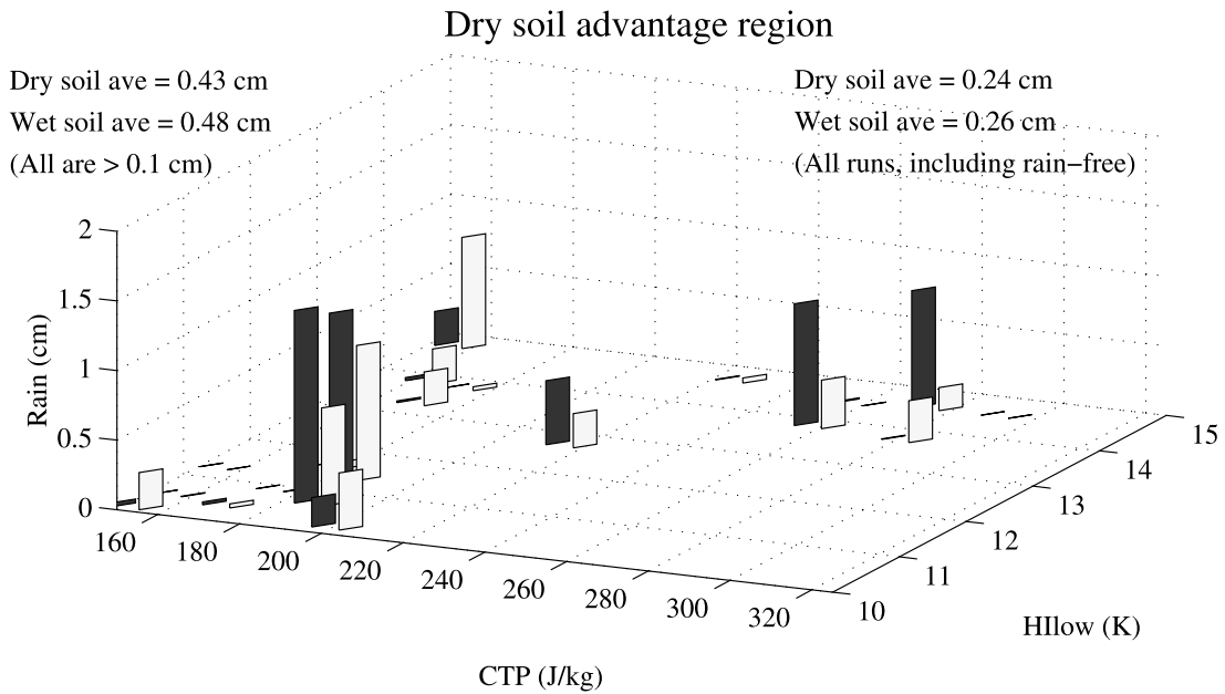
Figure 12. Outcome of the MM5 simulations with initial conditions falling in the dry soil advantage regime. Symbols in the top plot are as in Figure 4.
