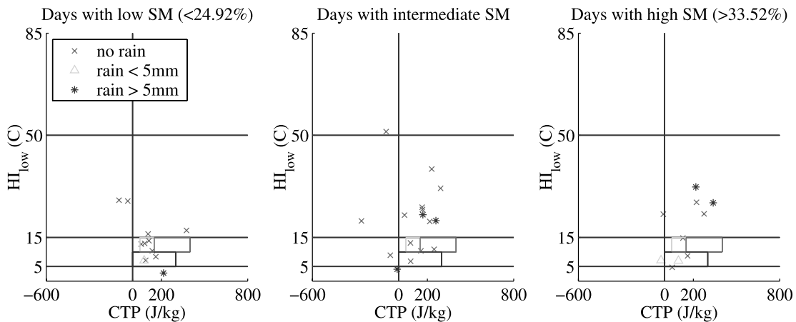
Figure 15. CTP, HI_{low} , and area-average rainfall for days with (left) low, (middle) intermediate, and (right) high soil moisture. Crosses indicate no rain, triangles indicate rain < 5 mm, and stars indicate rain > 5 mm.
