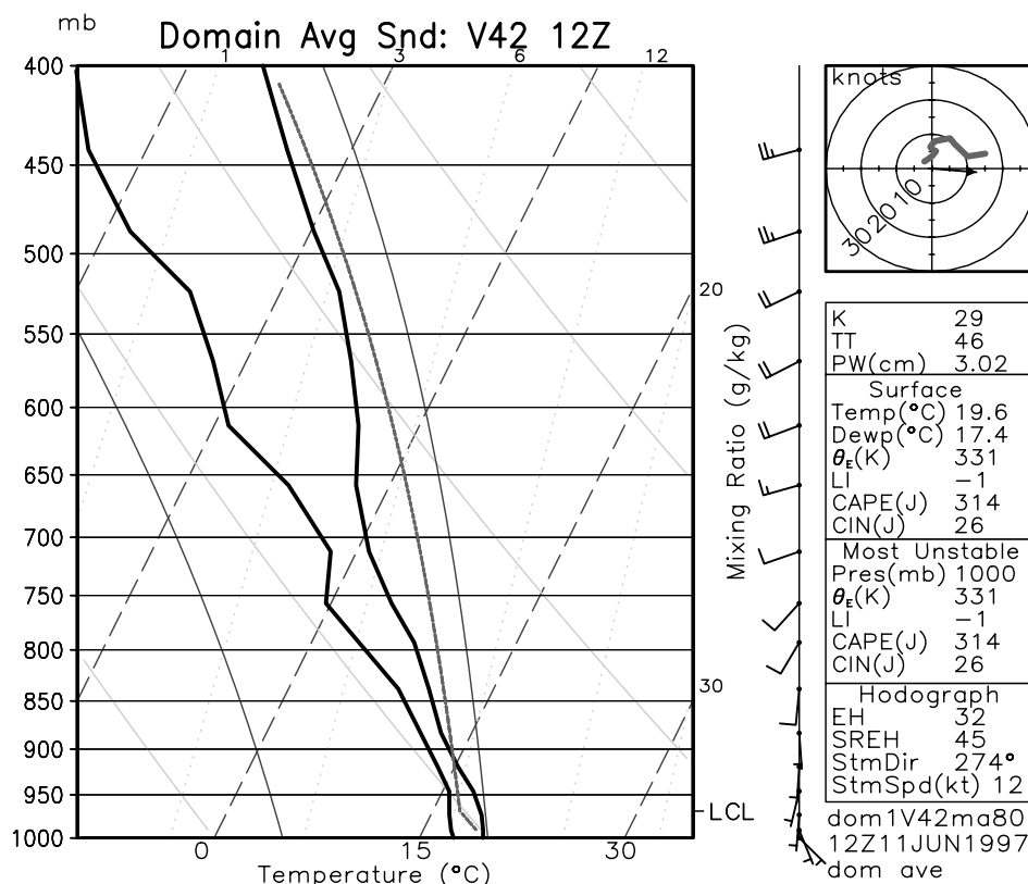
Figure 6. Initial domain average sounding for run V42 on a thermodynamic diagram. Thick solid lines are the temperature and dew point temperature profiles; thin solid lines are dry adiabats (constant potential temperature); dashed lines are constant temperature; dotted lines are constant mixing ratio; solid shaded lines are moist adiabats (constant equivalent potential temperature); and the solid line originating near the surface between the solid lines marks the trajectory of a lifted surface parcel. The hodograph tracks the winds in the lowest 300 mbar.
