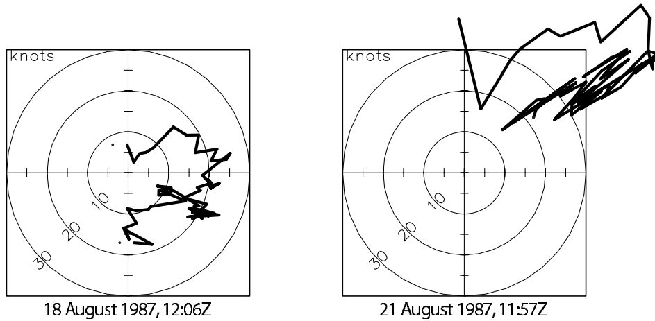
Figure 17. Hodographs (bottom 300 mbar) for 18 August 1987 (winds veer but stay under 30 knots; CTP = 217 J/kg; HI_{low} = 32^{\circ}C ; soil moisture = 37%; rain = 6.3 mm) and for 21 August 1987 (winds veer at speeds greater than 30 knots; CTP = 292 J/kg; HI_{low} = 32^{\circ}C ; soil moisture = 27%; rain = 0.0 mm).
