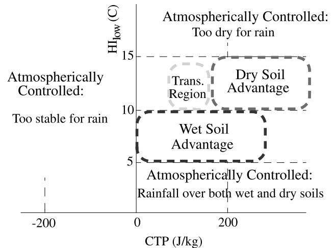
Figure 1. The CTP- HI_{low} framework for describing atmospheric controls on soil moisture-rainfall feedbacks. Only when the early morning atmosphere has CTP > 0 J/kg and 5 < HI_{low} < 15^{\circ}C can flux partitioning at the surface influence the triggering of convection. Trans Region is short for Transition Region.
