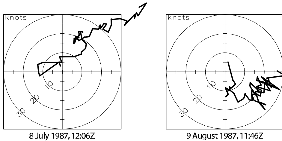
Figure 19. Hodographs (bottom 300 mbar) for 8 July 1987 (rain = 0.07 mm; strong low-level shear; CTP = 247 J/kg; HI_{low} = 11^{\circ}\text{C} ; soil moisture = 33%) and for 9 August 1987 (rain = 0.0 mm; strong low-level backing of the winds; CTP = -58 J/kg; HI_{low} = 9^{\circ}\text{C} ; soil moisture = 30%).
