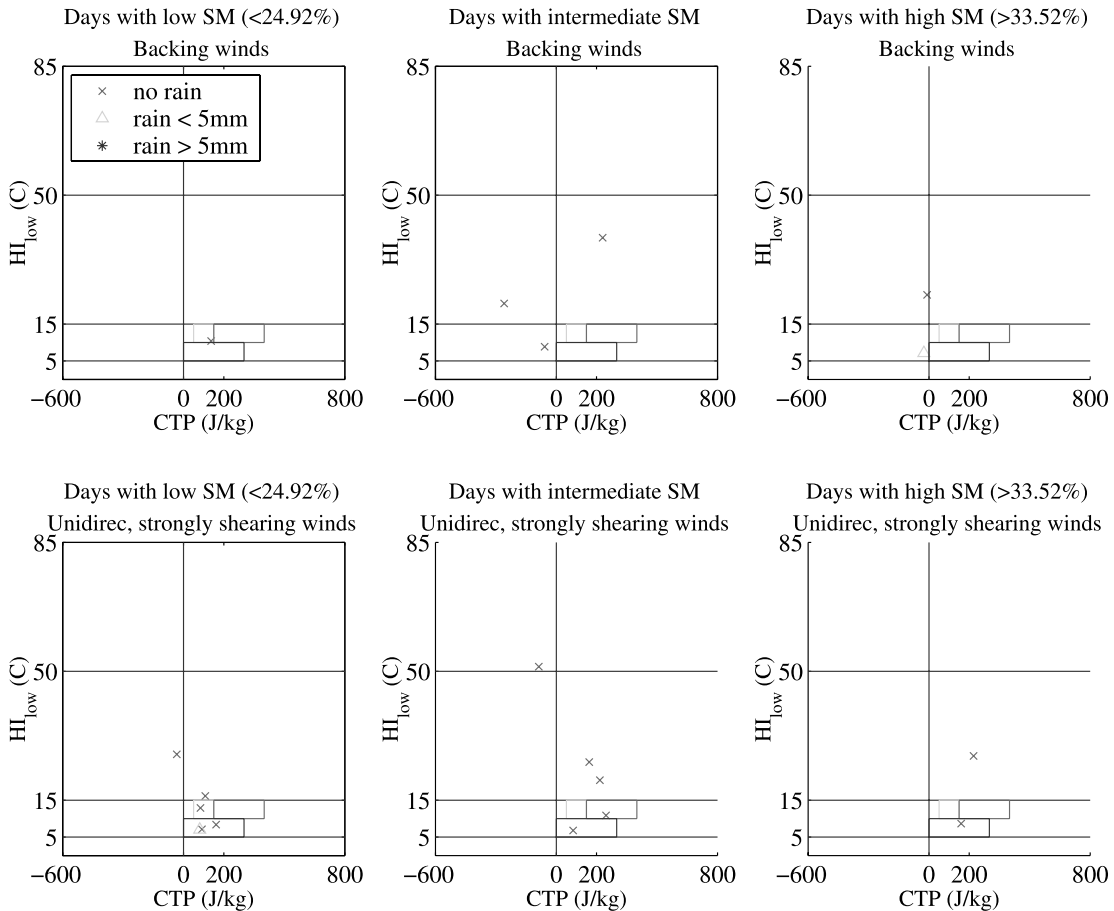
Figure 18. As in Figure 15 but only for those days with (top) backing or (bottom) strongly shearing unidirectional winds.
