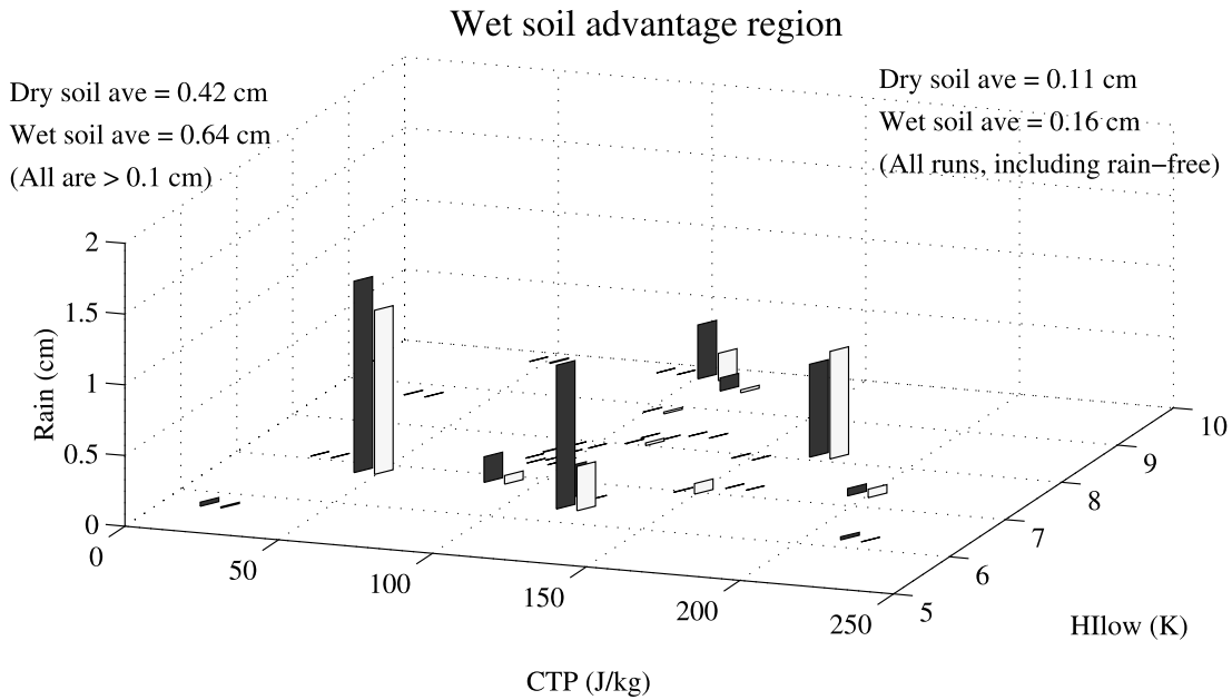
Figure 9. Outcome of the MM5 simulations with initial conditions falling in the wet soil advantage regime. Symbols in the top plot are as in Figure 4.
