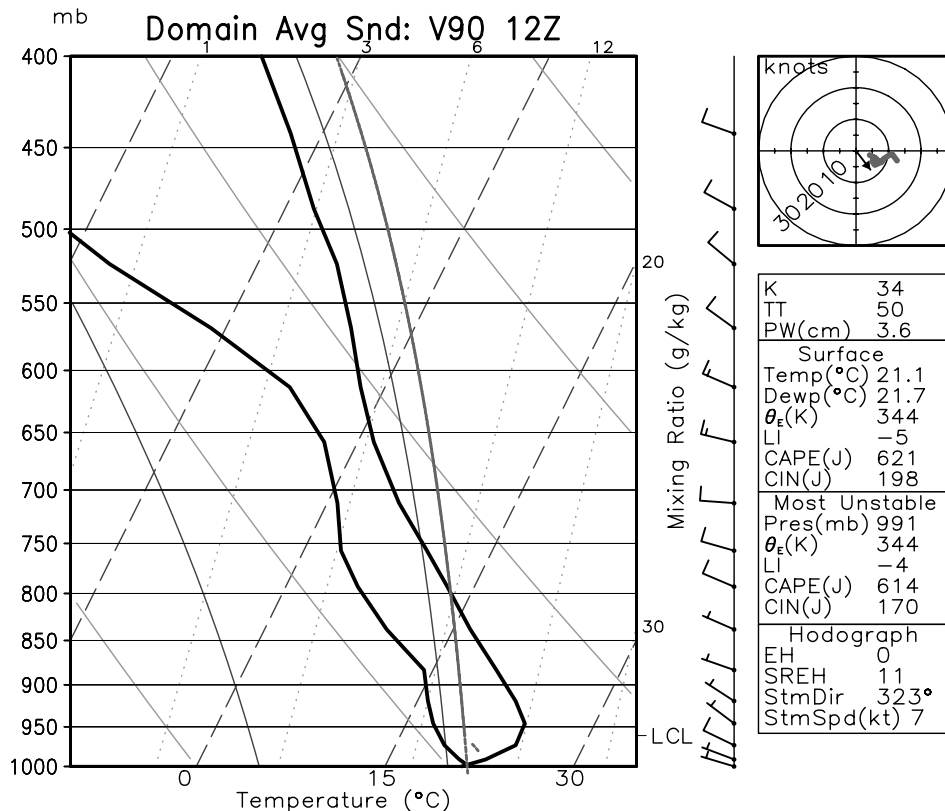
Figure 13. As in Figure 6 but for run V90.
