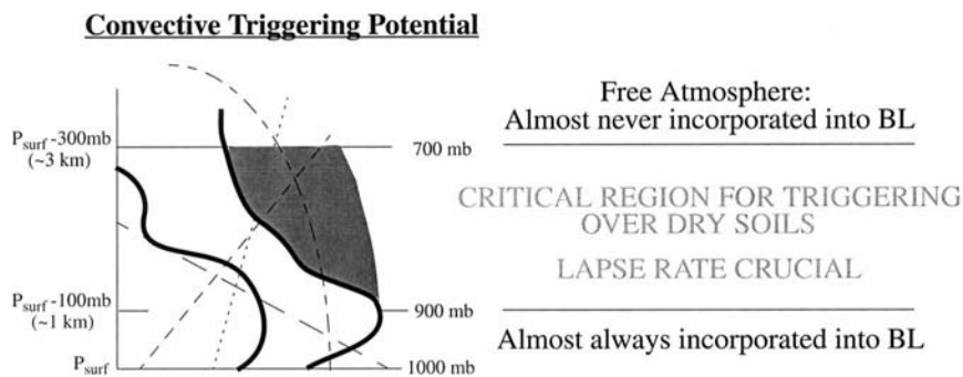
FIG. A1. A sketch of the definition of the convective triggering potential on a thermodynamic diagram. Thick solid lines are the temperature and dewpoint temperature profiles; straight long-dashed line is a dry adiabat (constant potential temperature); straight short-dashed line is constant temperature; straight dotted line is constant mixing ratio; curved short-dashed line is a moist adiabat (constant equivalent potential temperature). The CTP is determined by integrating the area between the observed temperature sounding and a moist adiabat originating at the observed temperature 100 mb above the surface. The top is bounded by a constant pressure line 300 mb above the surface. Note that the CTP can be negative if the value of the moist adiabat originating from the P_{surf}-100 -mb level is less than the observed equivalent potential temperatures at higher levels. Also, the CTP will be zero if the observed profile is moist adiabatic above the point of origin. (Figure reprinted from Findell and Eltahir 2003b.)
