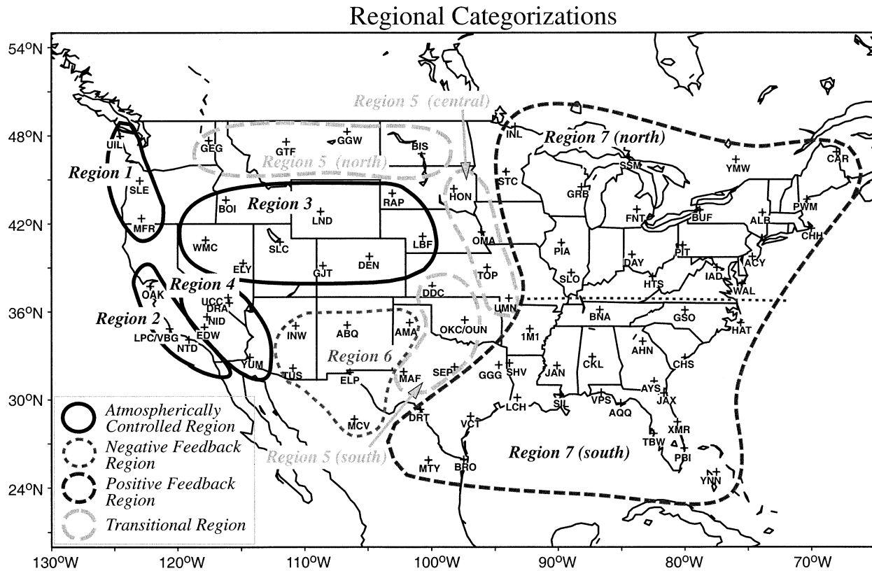
FIG. 2. Representative regions within the continental United States, based on CTP- HI_{low} scatterplots for the 89 stations with at least 10 yr of data during 1957–98 (see text for full description).
