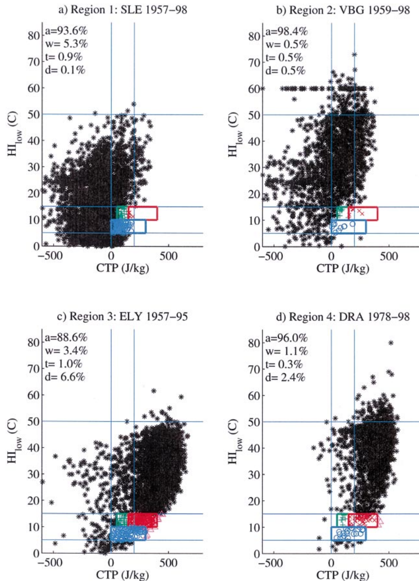
FIG. 4. Early-morning CTP and HI_{low} for all available soundings from Jun, Jul, and Aug 1957–98 from representative stations in (a) region 1, the Pacific Northwest (SLE: Salem, OR); (b) region 2, the Pacific southwest (VBG: Vandenberg, CA); (c) region 3, the central Rocky Mountains (ELY: eastern-central NV); and (d) region 4, the dry intermontane region (DRA: Desert Rock, NV). In the legends, a is the percentage of atmospherically controlled days (black star); w is the percentage of days in the wet soil advantage regime (blue circle); t is the percentage of days in the transition region (green cross); and d is the percentage of days in the dry soil advantage regime (red x). Pink triangles are outside the regions of CTP- HI_{low} space defined by earlier analyses (less than 1% in each case).
