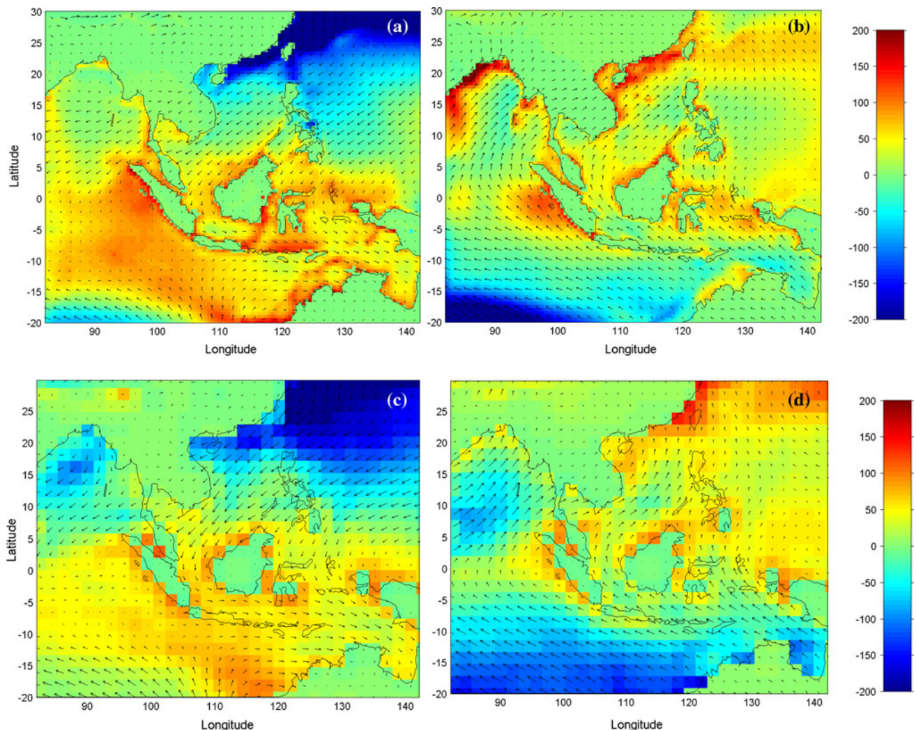
Fig. 3 Decadal average (1970s) coupled simulation of heat flux and winds for a winter and b summer. The wind vectors are shown every 100 km. NCEP heat fluxes and winds are shown in c winter and d summer for comparison
