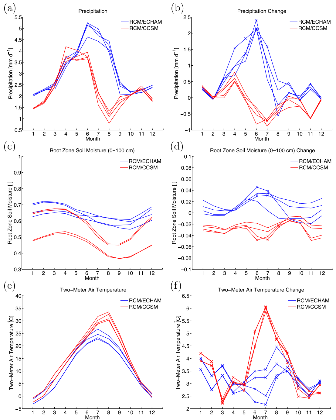
Figure 4. Simulated historical seasonal cycles and future changes in seasonal cycles of precipitation, soil moisture, and surface temperature. RCM historical (1984–2005) seasonal cycles of: (a) precipitation, (c) root zone soil moisture, and (e) 2 m air temperature averaged over the box in Figure 3. Differences between RCM future (2078–2099) and historical (1984–2005) seasonal cycles of: (b) precipitation, (d) root zone soil moisture, and (f) 2 m air temperature averaged over the box in Figure 3. Crosses denote nonoverlapping 95% confidence intervals between future and historical seasonal cycles. Line color denotes lateral boundary condition; convective parameterization (FC, AS) and land surface scheme (IBIS, BATS) are not differentiated.
