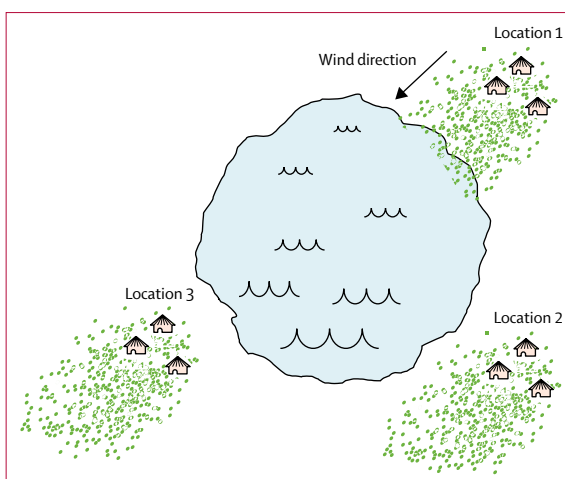
Figure 6: Schematic of the role of wind for different village locations
