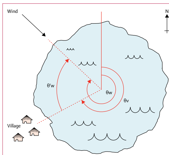
Figure 2: Definition of wind direction
