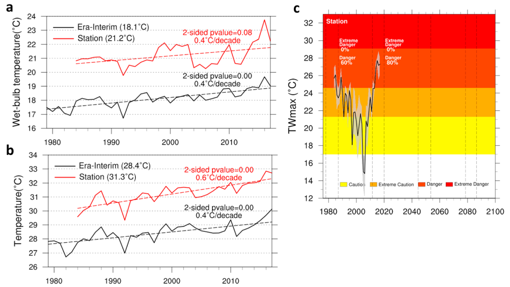
Figure 2. Time series of annual mean (a) TW and (b) T and (c) daily TW_{max} ( ^{\circ}C ) during Hajj. In (a) and (b), station and ERA-Interim data with trendlines are indicated in red for the period 1984–2017 and black for 1979–2017, respectively, and the values represent the average, two-sided Mann-Kendall p values, and decadal trend. In (c), the black line represents the 5-day TW_{max} average of the station observations during Hajj; shading indicates the maximum and minimum; background colors indicate U.S. National Weather Service heat stress risk level equivalents at 45% relative humidity in Figure S8; and vertical dashed lines indicate bounds of Hajj periods occurring during August through October.
