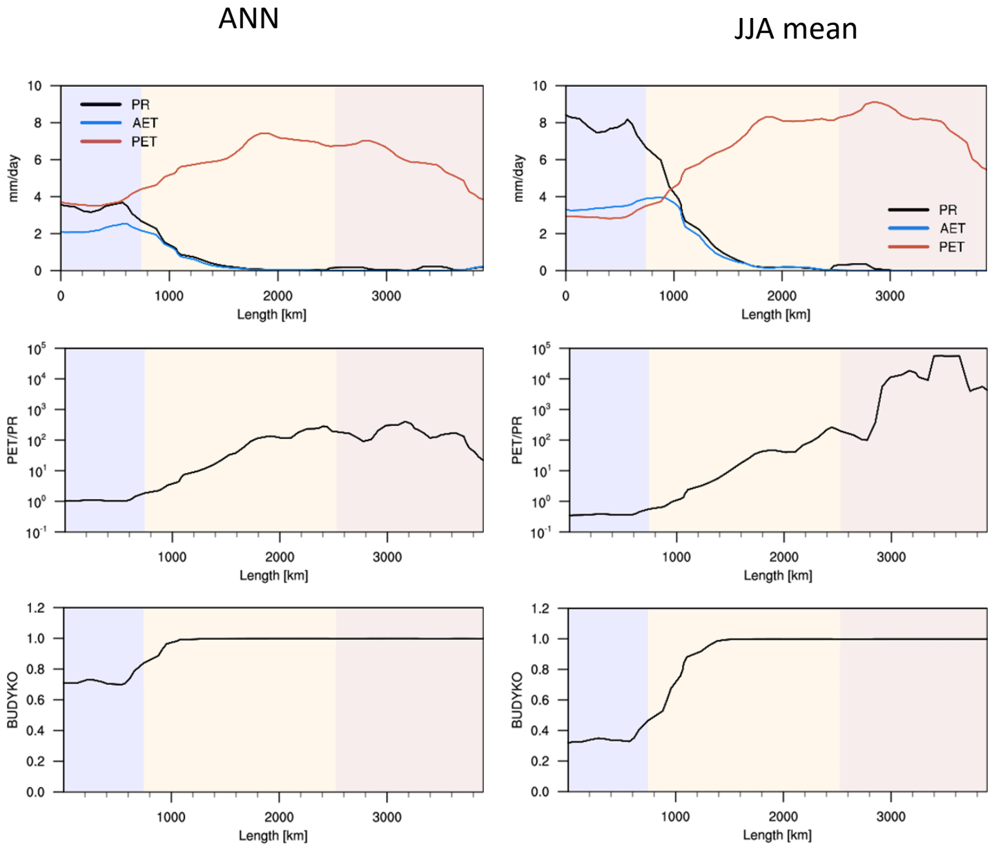
Figure 6: Application of the theory in the Nile basin. Walking down the river from Lake Tana to Mediterranean (ANN is annual; JJA is June, July, August) PR: precipitation; AET: Actual evapotranspiration; PET: Potential evapotranspiration; Blue: Ethiopia, Yellow: Sudan, red: Egypt
